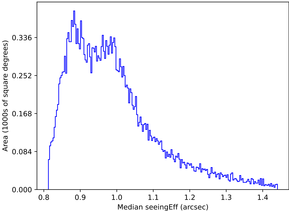
weather_cloudso16v3.4_10yrs Yr 1 all bands: Median seeingEff
