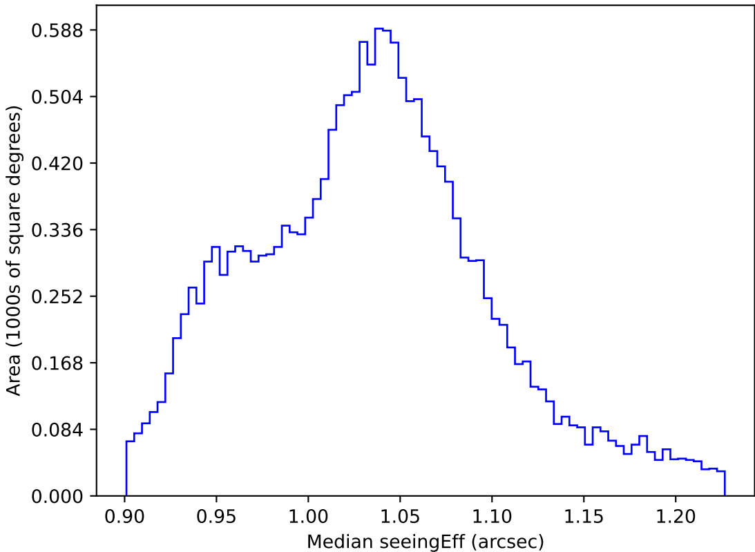
weather_cloudso16v3.4_10yrs WFD z band: Median seeingEff
