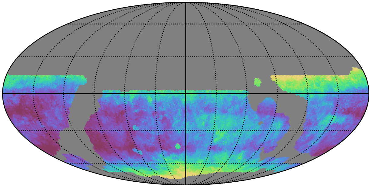
weather_cloudso16v3.4_10yrs WFD r band: Median seeingEff
