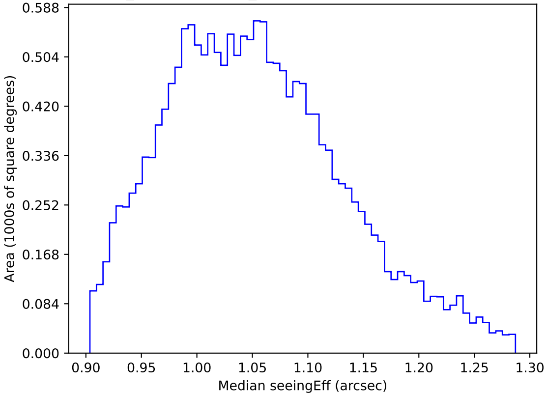
weather_cloudso16v3.4_10yrs WFD r band: Median seeingEff
