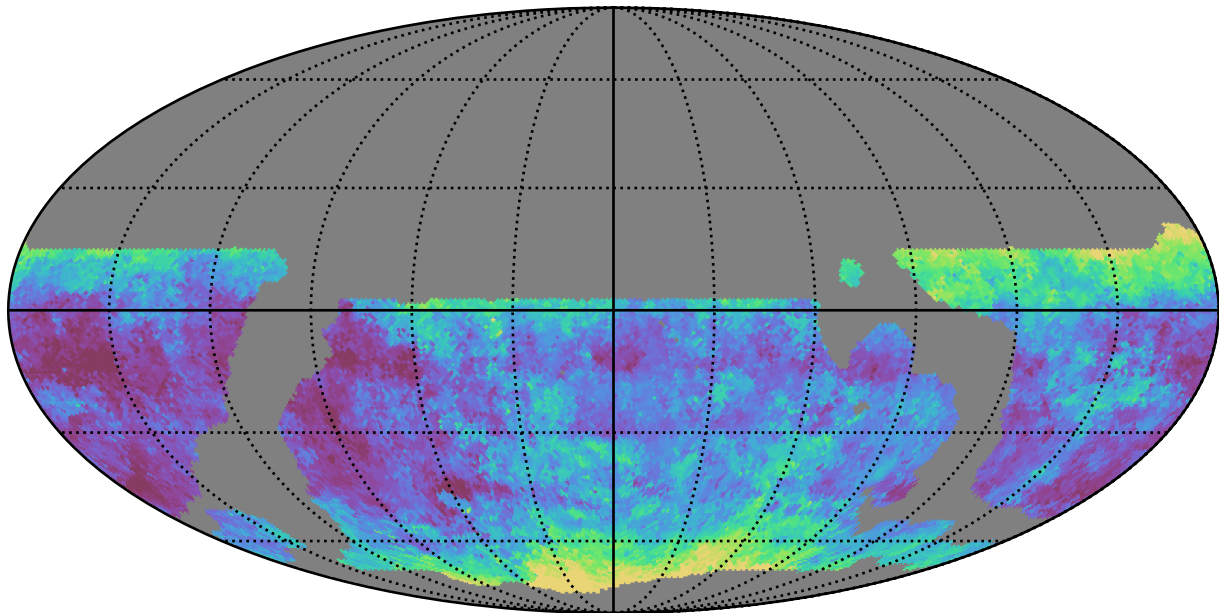
weather_cloudso16v3.4_10yrs WFD g band: Median seeingEff
