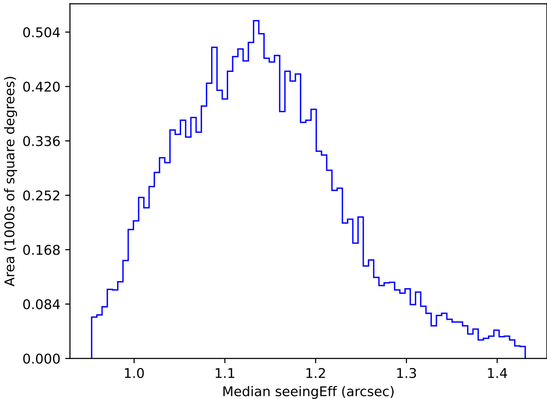
weather_cloudso16v3.4_10yrs WFD g band: Median seeingEff
