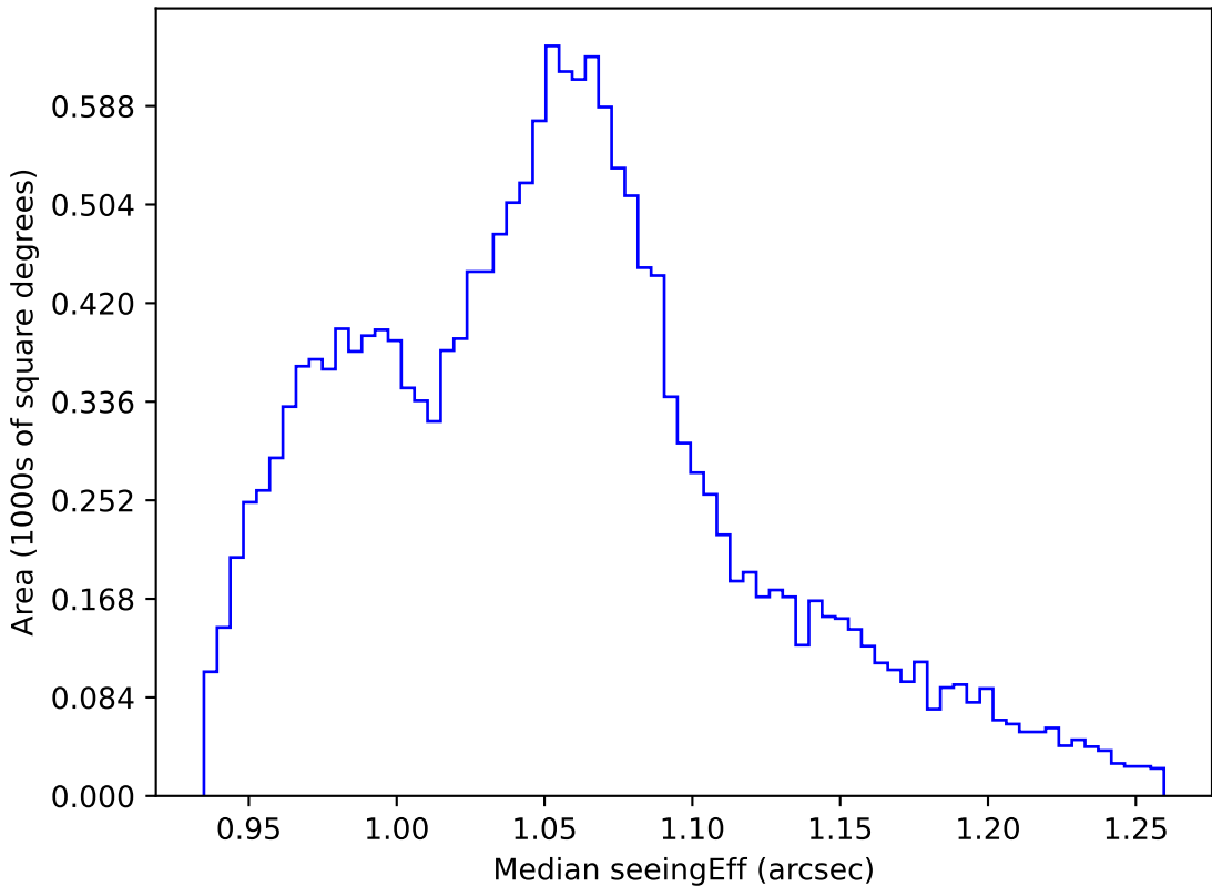
weather_cloudso16v3.4_10yrs WFD all bands: Median seeingEff
