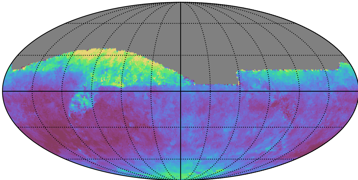
weather_cloudso16v3.4_10yrs All sky z band: Median seeingEff
