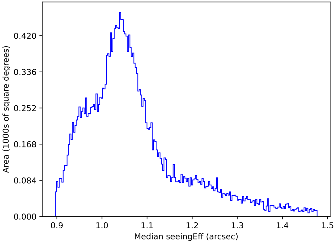
weather_cloudso16v3.4_10yrs All sky z band: Median seeingEff
