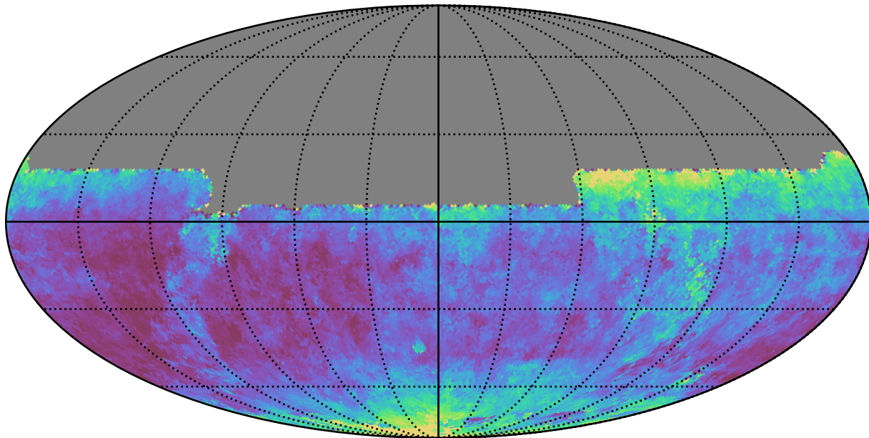
weather_cloudso16v3.4_10yrs All sky y band: Median seeingEff
