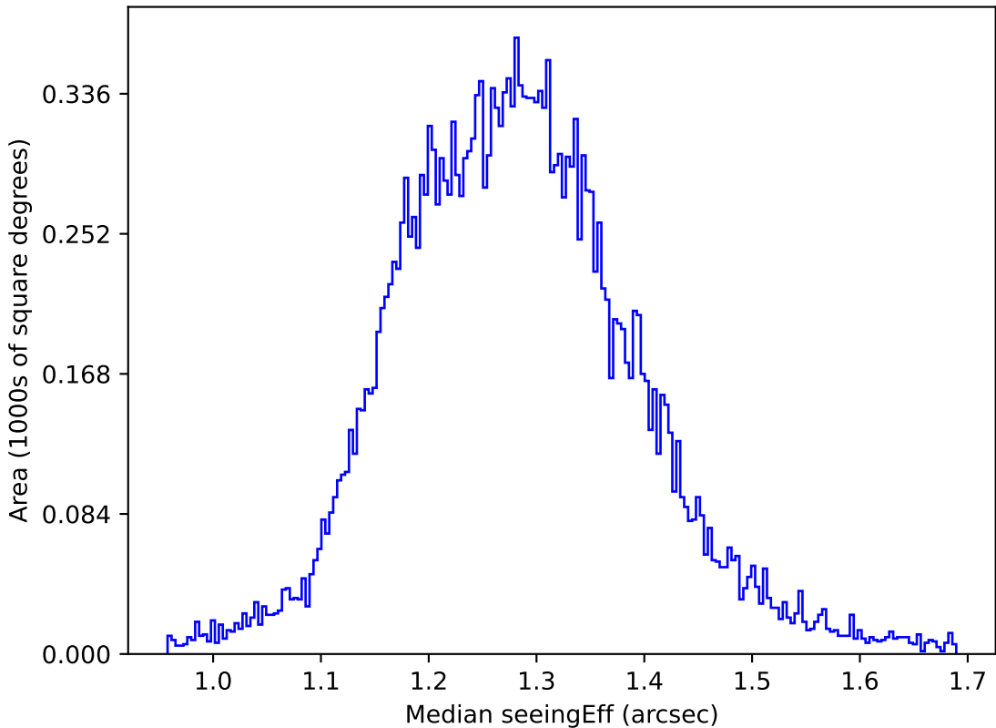
weather_cloudso16v3.4_10yrs All sky u band: Median seeingEff
