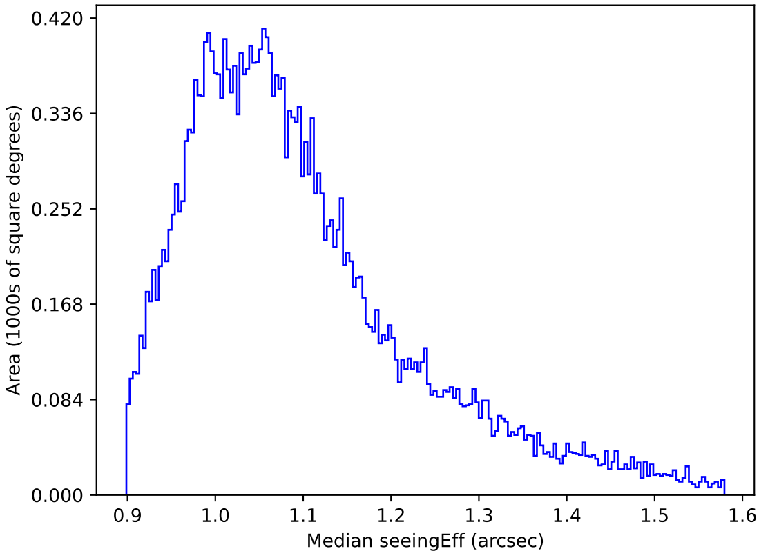
weather_cloudso16v3.4_10yrs All sky r band: Median seeingEff
