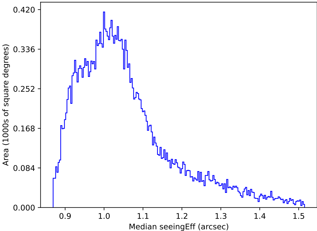
weather_cloudso16v3.4_10yrs All sky i band: Median seeingEff
