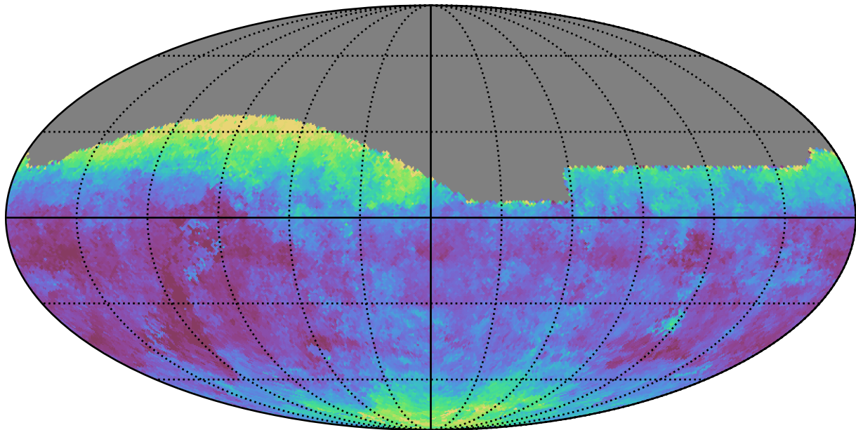
weather_cloudso16v3.4_10yrs All sky g band: Median seeingEff
