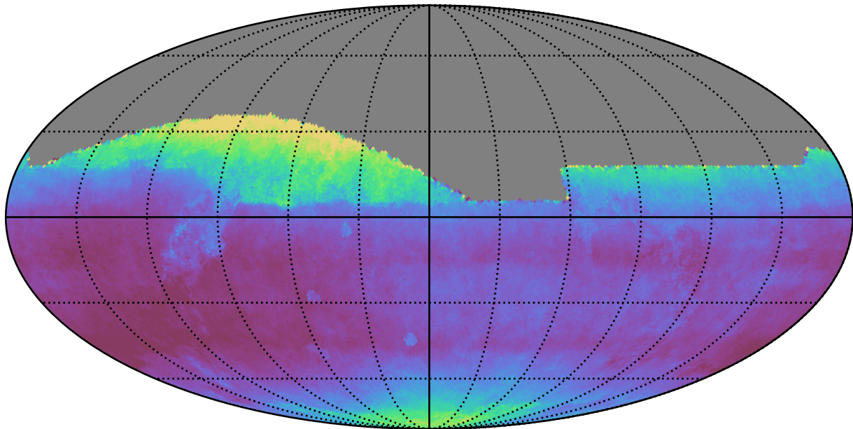
weather_cloudso16v3.4_10yrs All sky all bands: Median seeingEff
