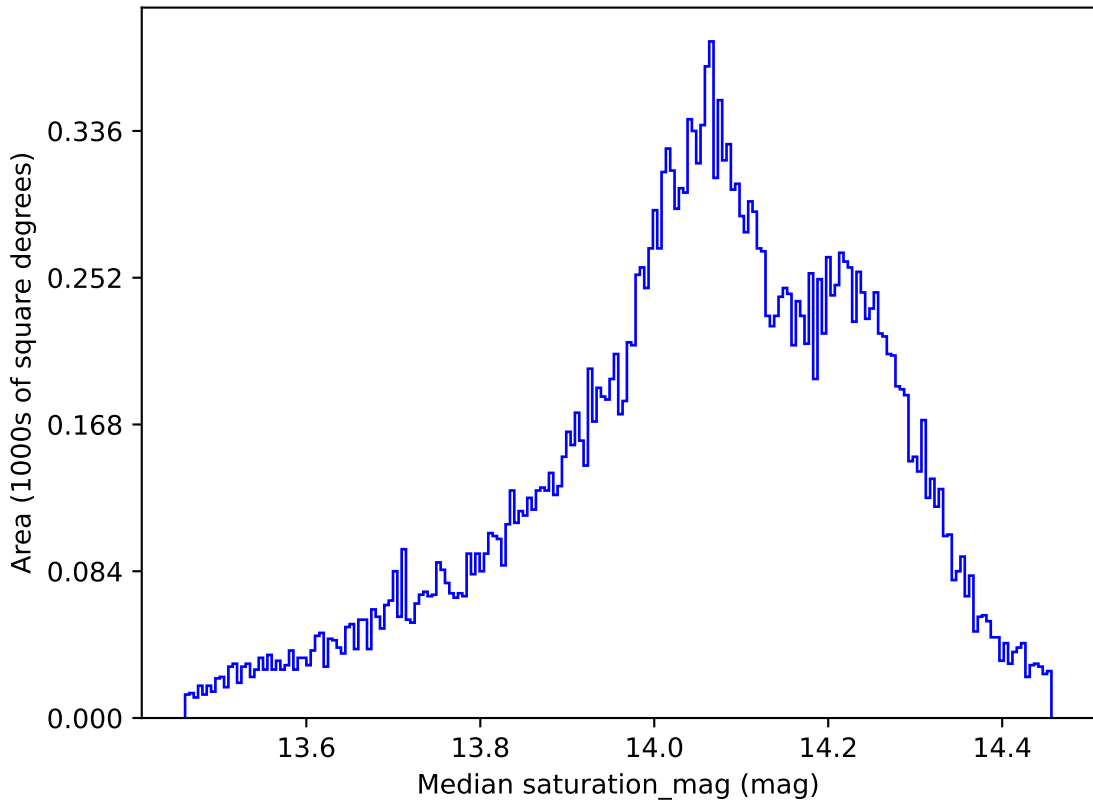
weather_cloudso16v3.4_10yrs All sky all bands: Median saturation_mag
