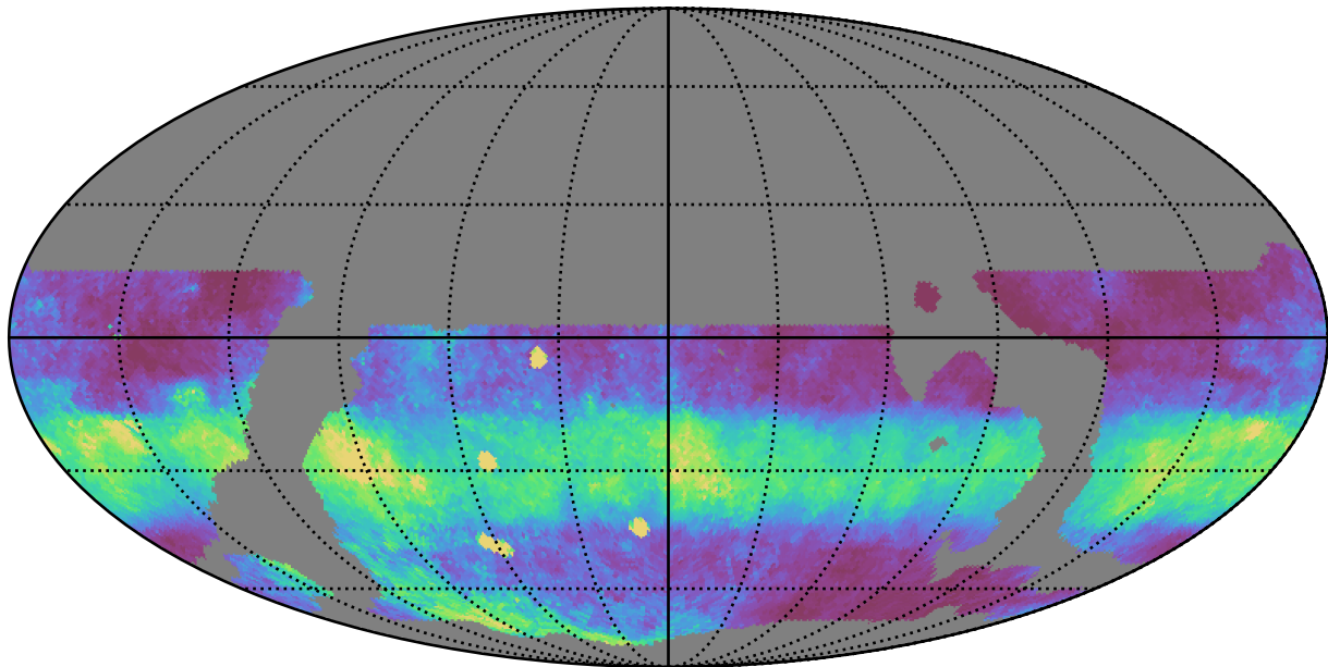
weather_cloudso16v3.4_10yrs WFD z band: Median normairmass
