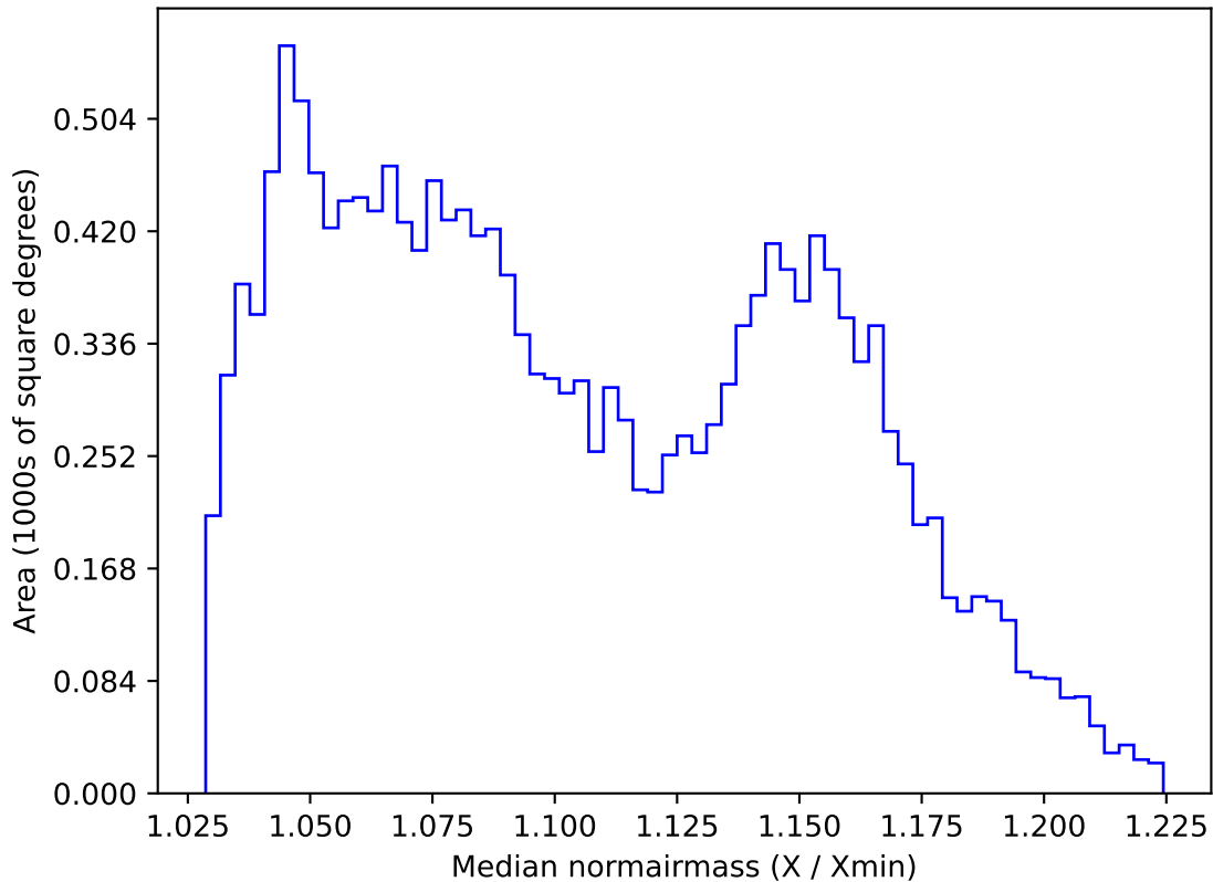
weather_cloudso16v3.4_10yrs WFD z band: Median normairmass
