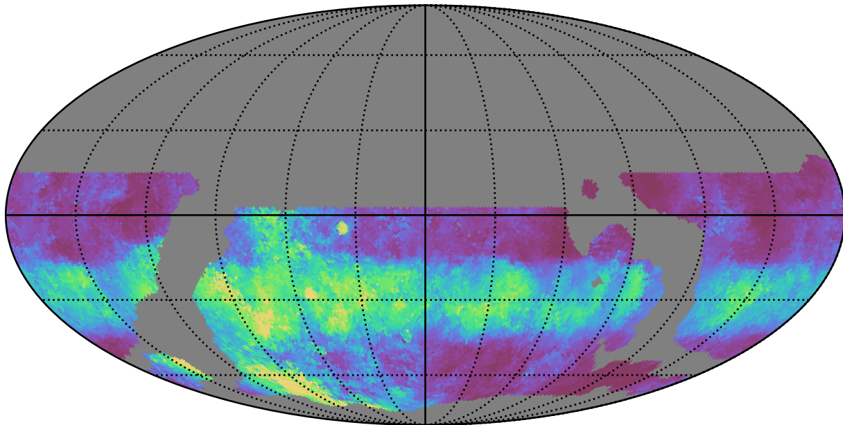
weather_cloudso16v3.4_10yrs WFD u band: Median normairmass
