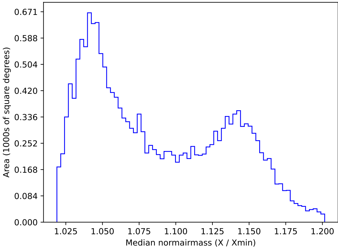
weather_cloudso16v3.4_10yrs WFD r band: Median normairmass
