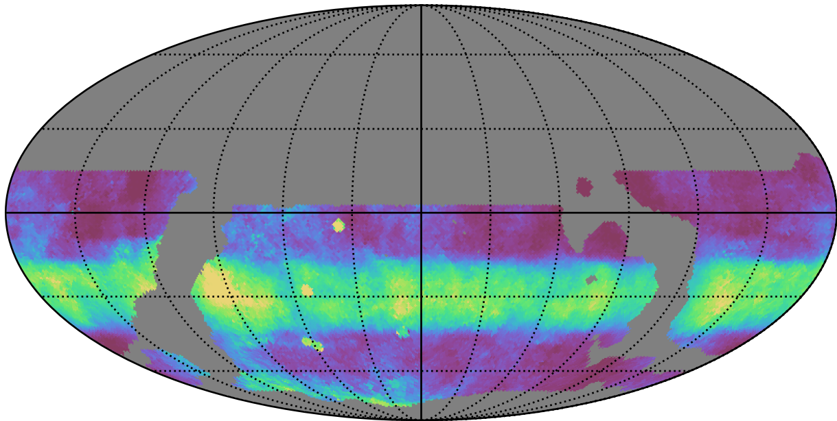
weather_cloudso16v3.4_10yrs WFD i band: Median normairmass
