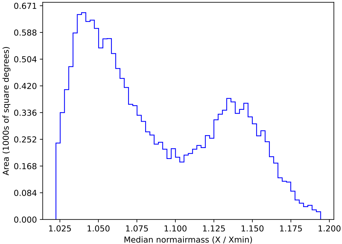
weather_cloudso16v3.4_10yrs WFD i band: Median normairmass
