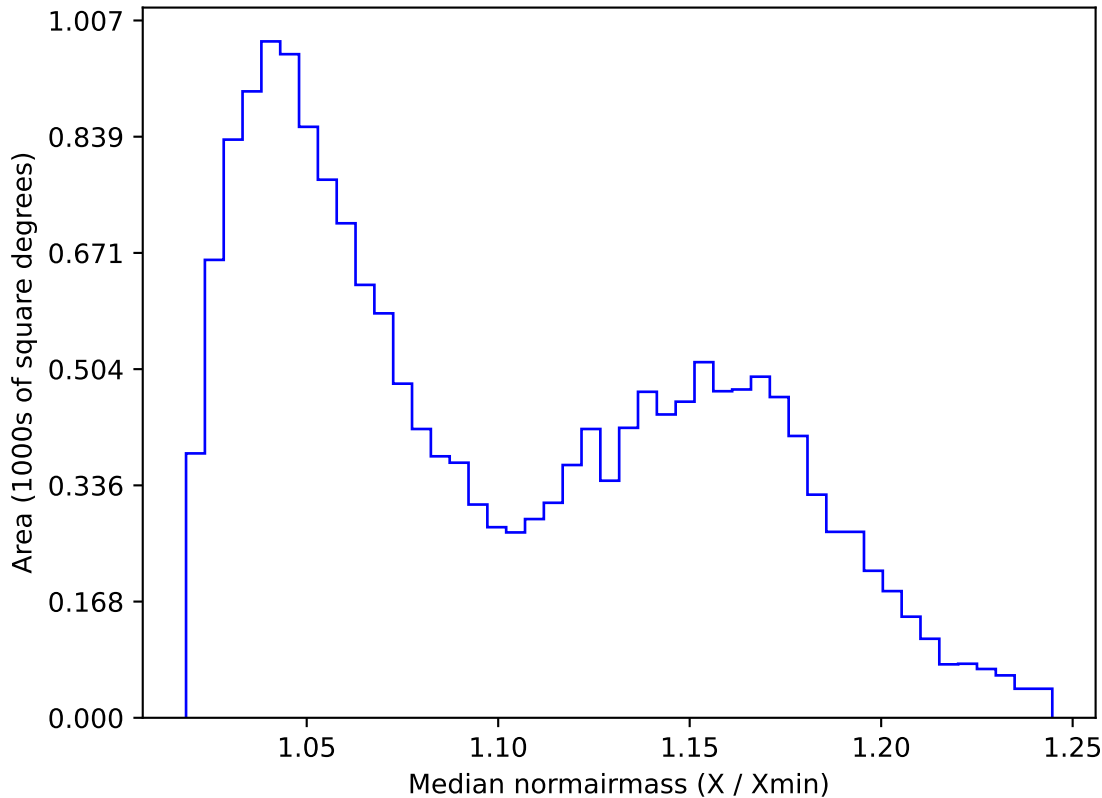
weather_cloudso16v3.4_10yrs WFD g band: Median normairmass
