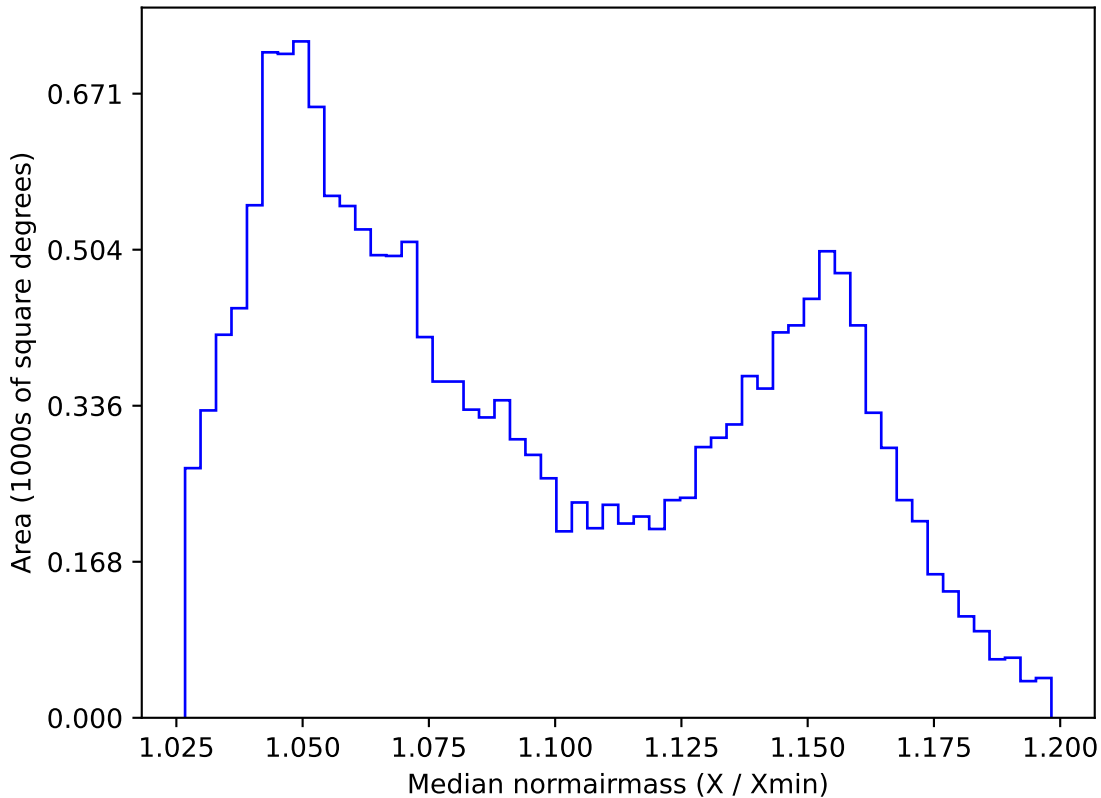
weather_cloudso16v3.4_10yrs WFD all bands: Median normairmass
