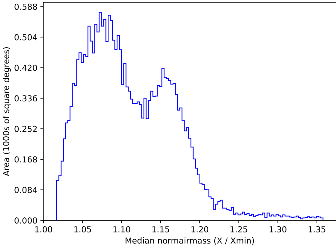
weather_cloudso16v3.4_10yrs All sky y band: Median normairmass
