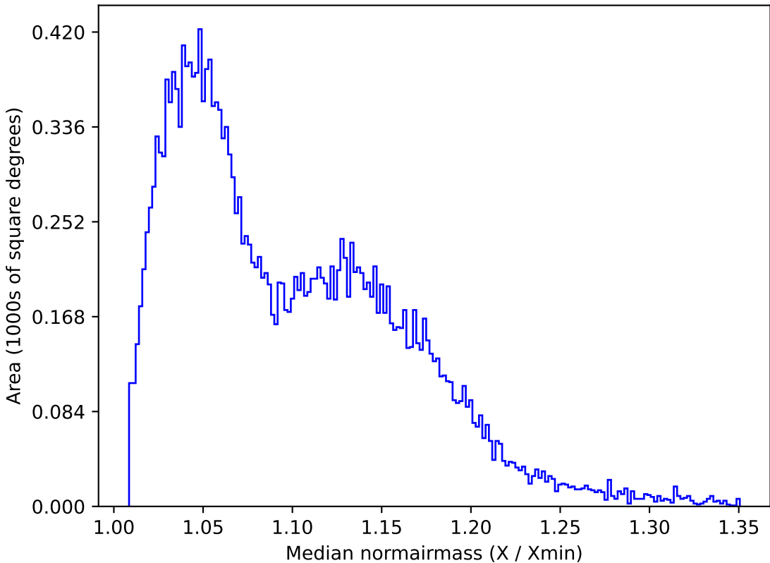
weather_cloudso16v3.4_10yrs All sky u band: Median normairmass
