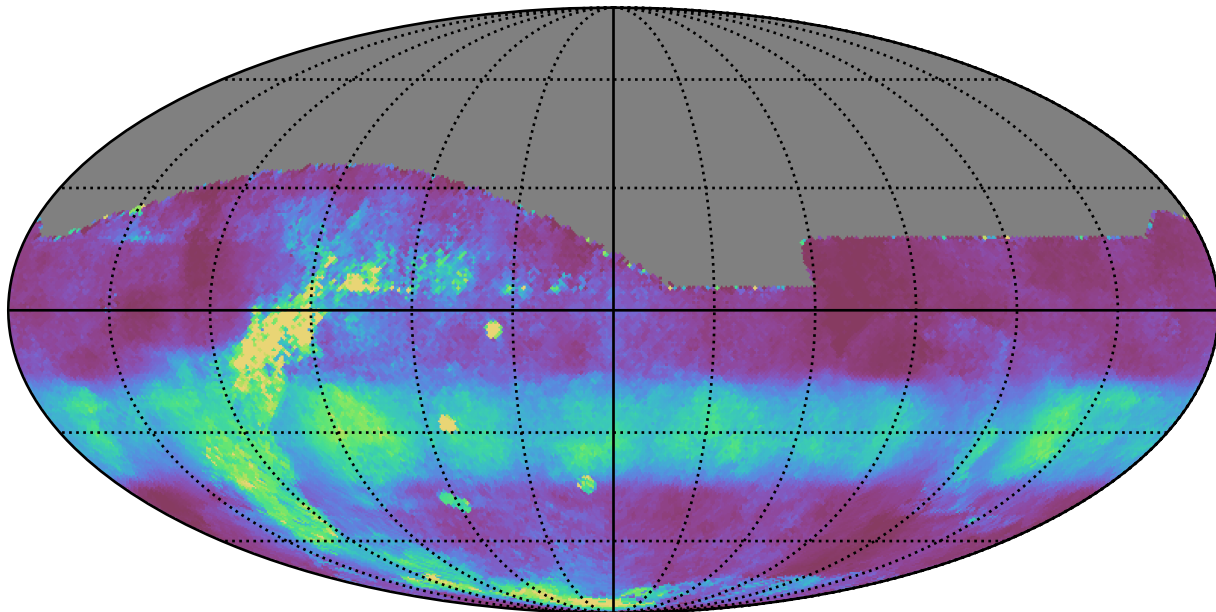
weather_cloudso16v3.4_10yrs All sky r band: Median normairmass
