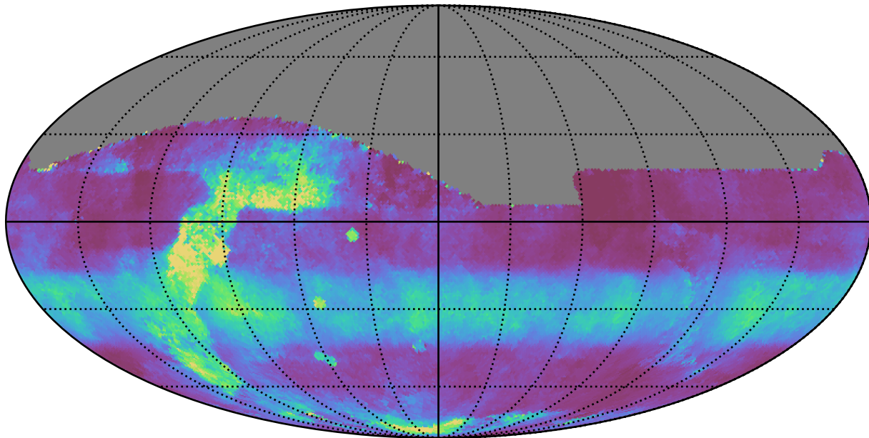
weather_cloudso16v3.4_10yrs All sky i band: Median normairmass
