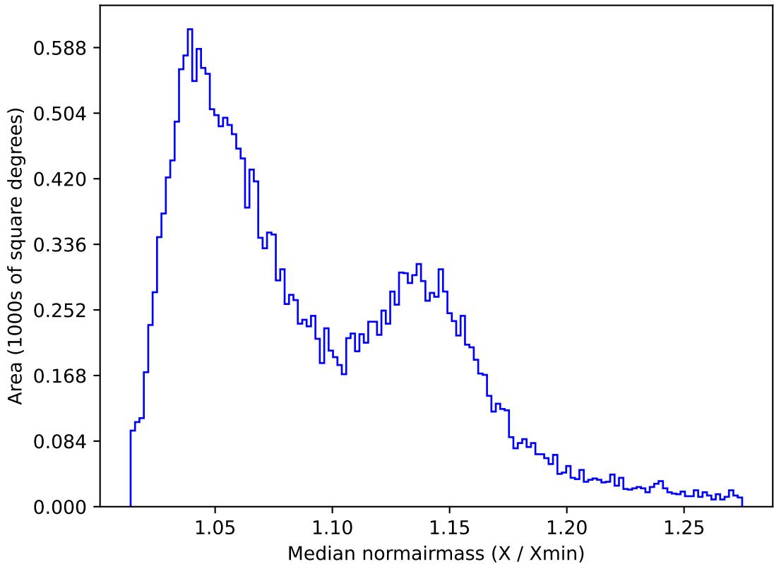
weather_cloudso16v3.4_10yrs All sky i band: Median normairmass
