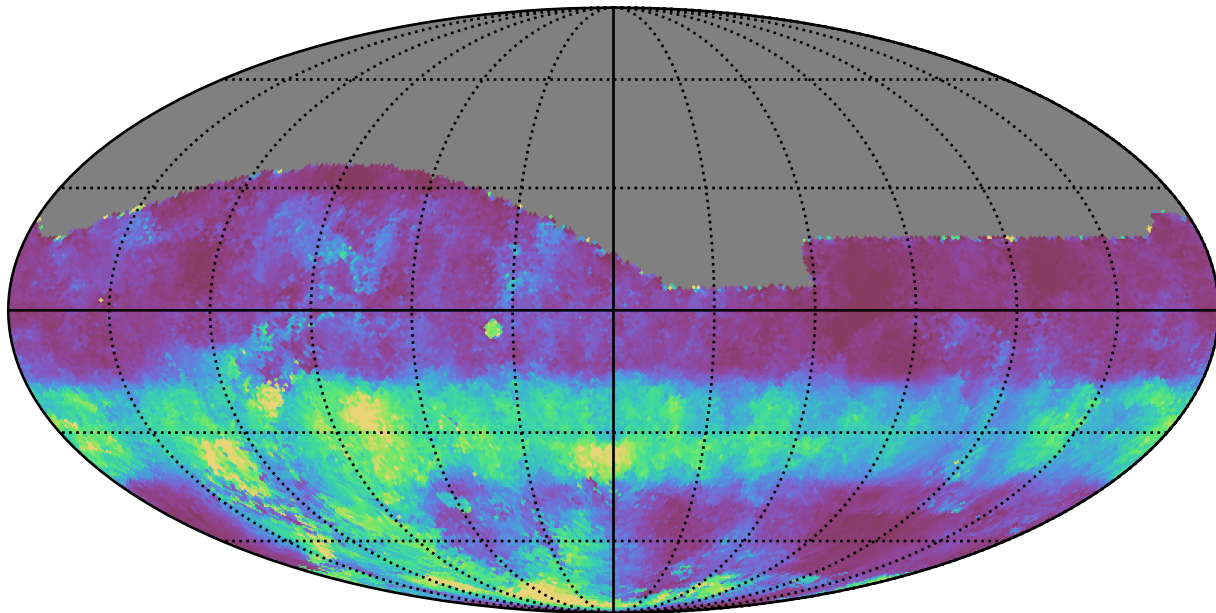
weather_cloudso16v3.4_10yrs All sky g band: Median normairmass
