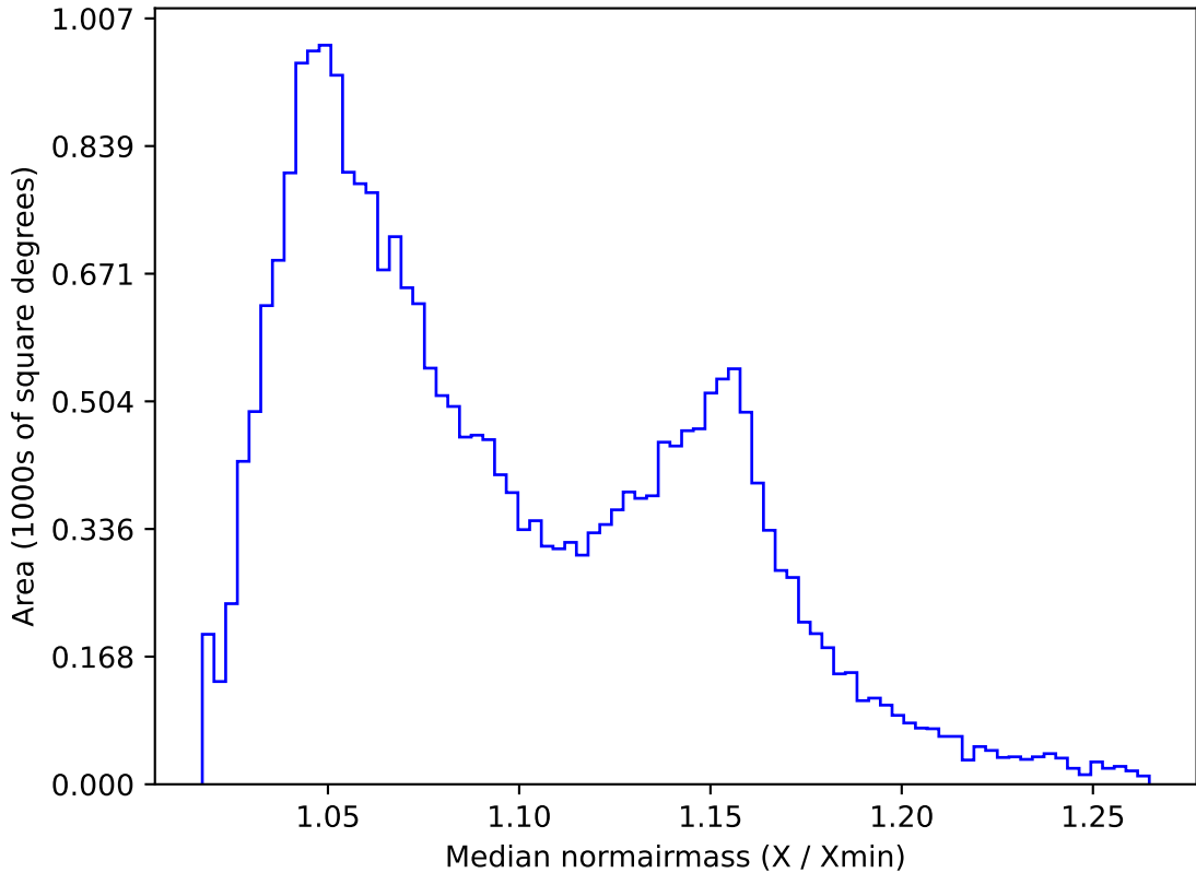
weather_cloudso16v3.4_10yrs All sky all bands: Median normairmass
