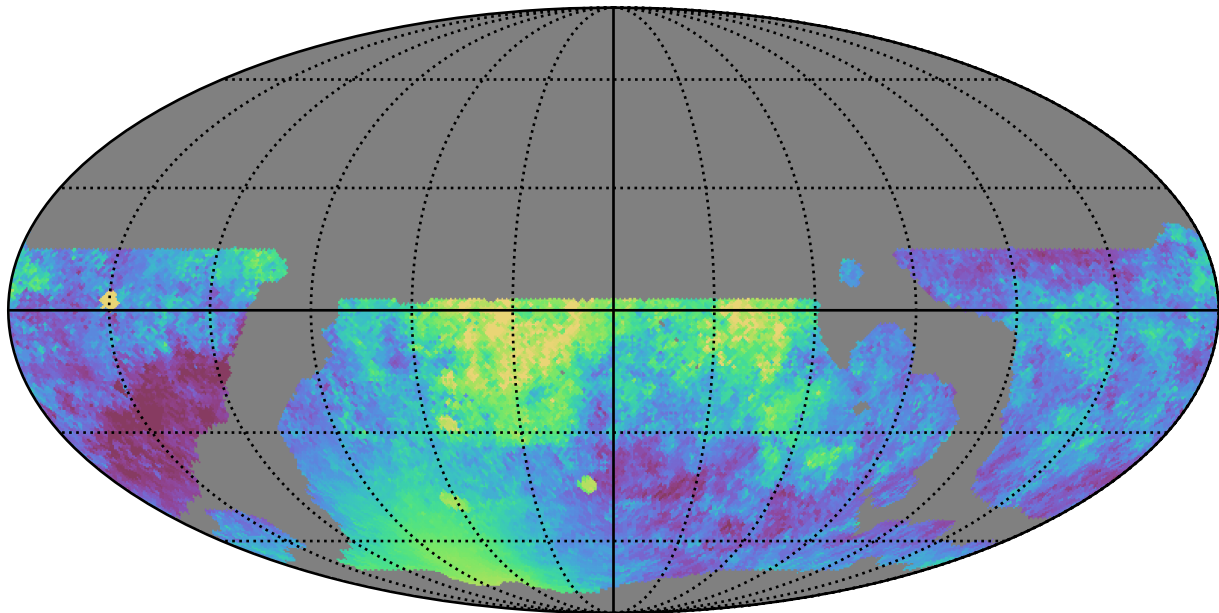
weather_cloudso16v3.4_10yrs WFD z band: Median moonDistance
