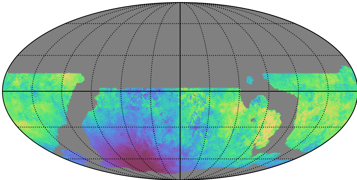
weather_cloudso16v3.4_10yrs WFD u band: Median moonDistance
