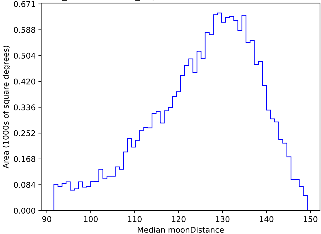
weather_cloudso16v3.4_10yrs WFD u band: Median moonDistance
