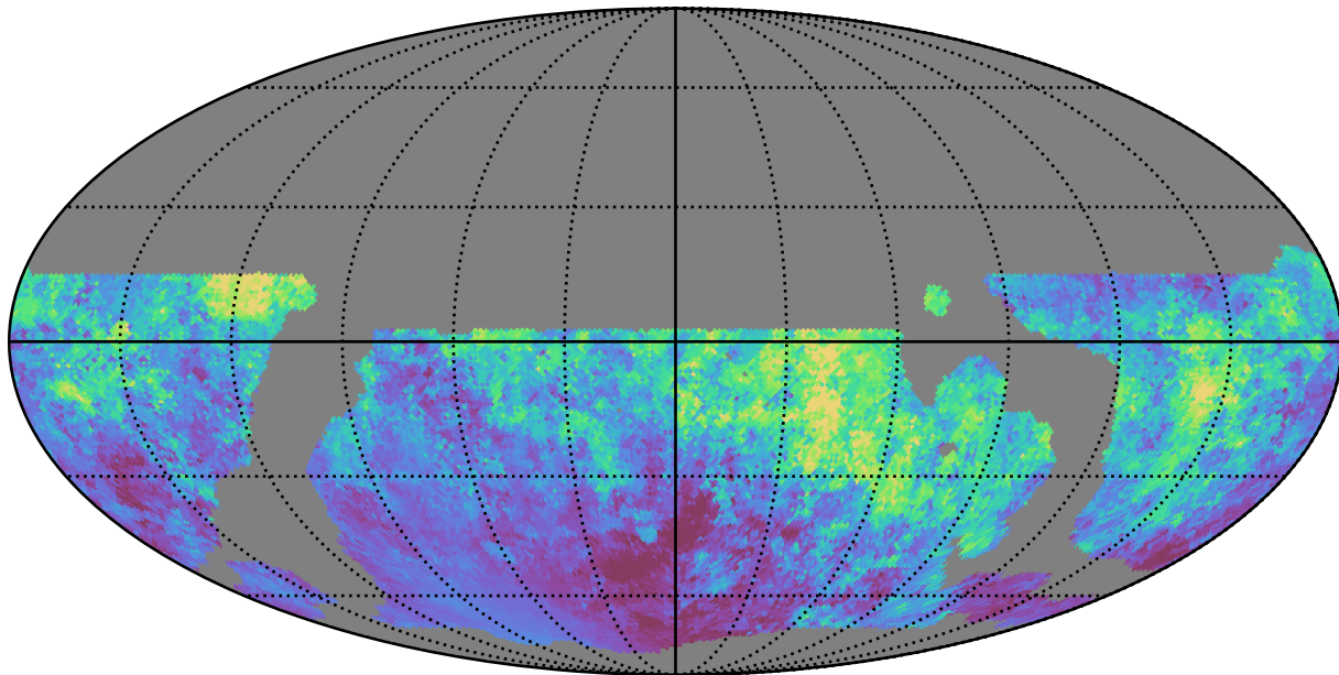
weather_cloudso16v3.4_10yrs WFD i band: Median moonDistance
