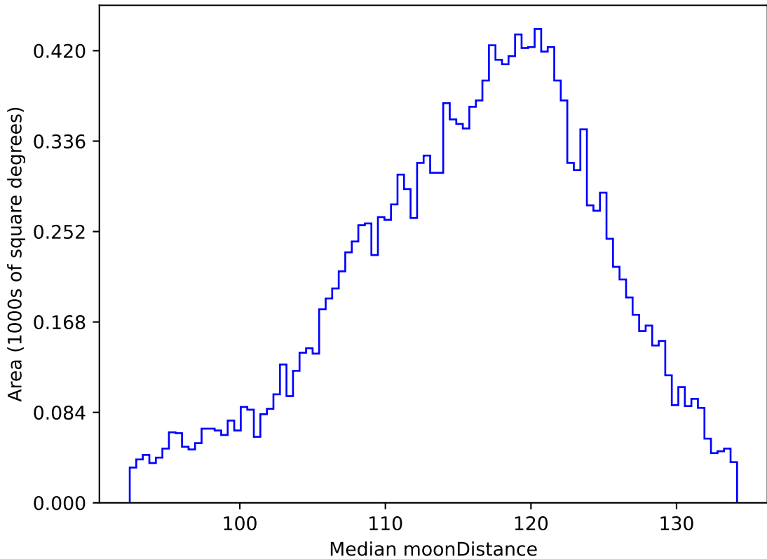
weather_cloudso16v3.4_10yrs WFD g band: Median moonDistance
