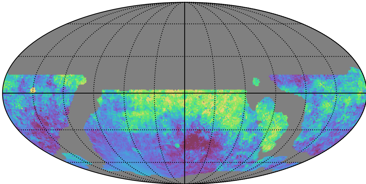
weather_cloudso16v3.4_10yrs WFD all bands: Median moonDistance
