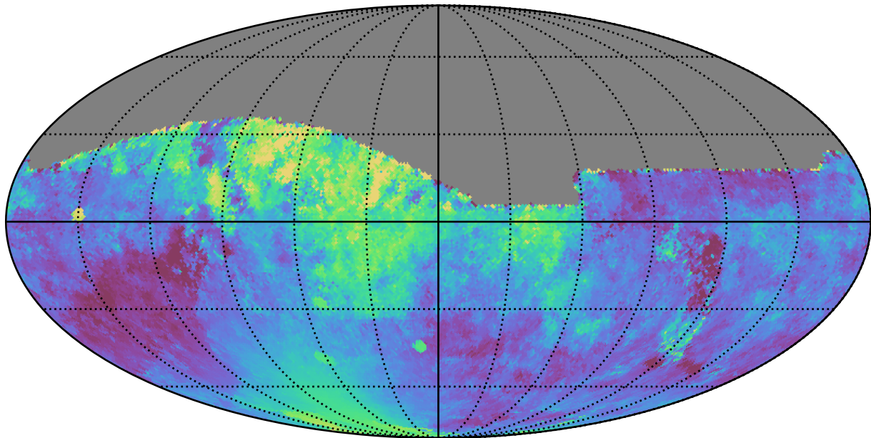
weather_cloudso16v3.4_10yrs All sky z band: Median moonDistance
