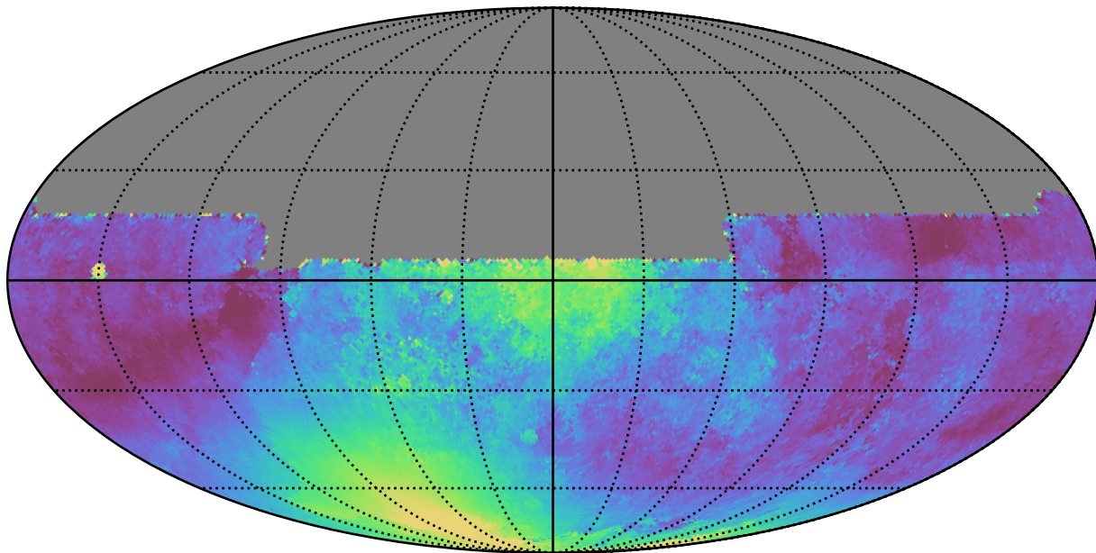
weather_cloudso16v3.4_10yrs All sky y band: Median moonDistance
