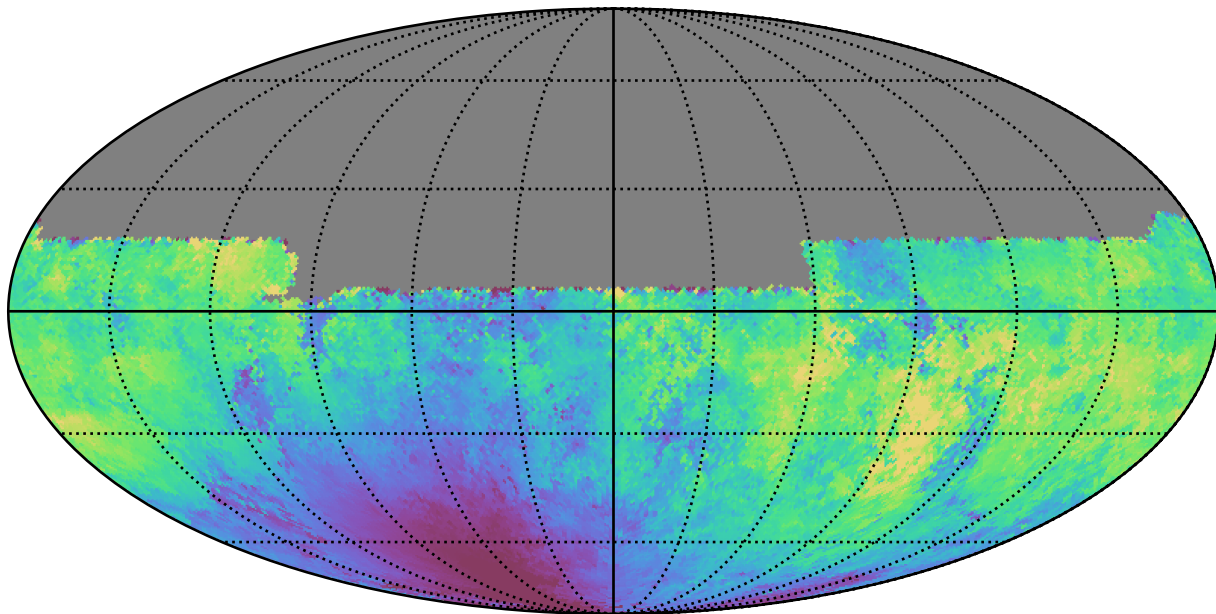
weather_cloudso16v3.4_10yrs All sky u band: Median moonDistance
