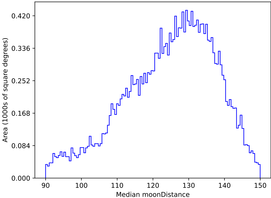
weather_cloudso16v3.4_10yrs All sky u band: Median moonDistance
