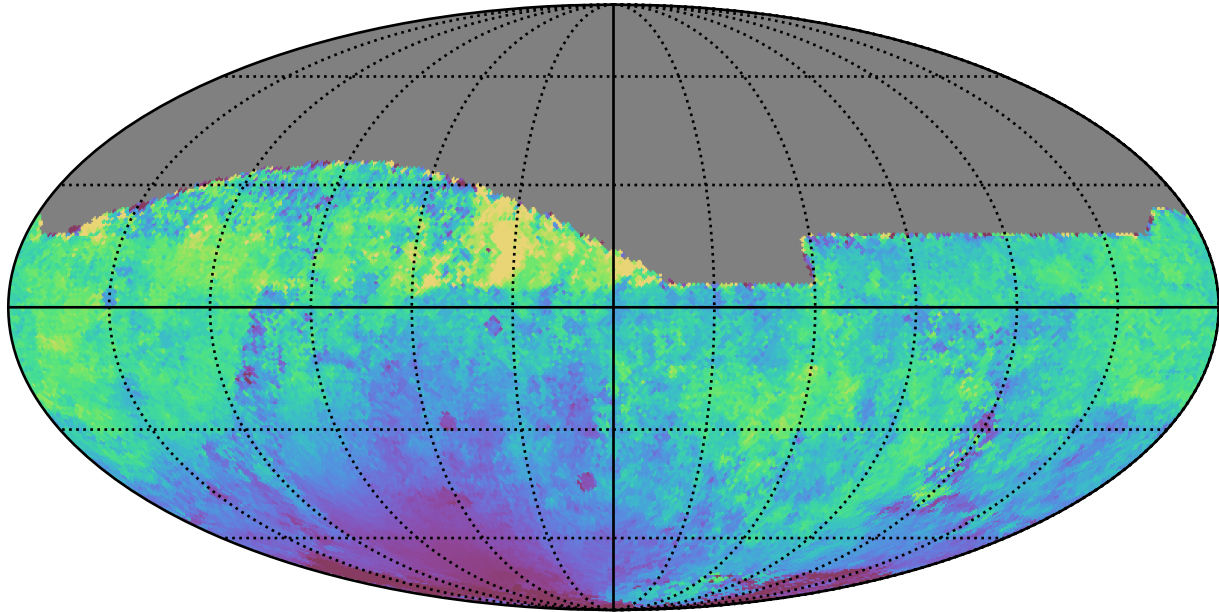
weather_cloudso16v3.4_10yrs All sky r band: Median moonDistance
