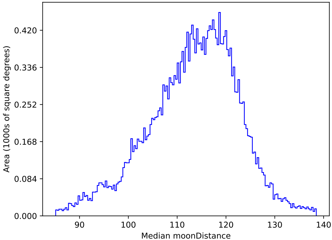
weather_cloudso16v3.4_10yrs All sky r band: Median moonDistance
