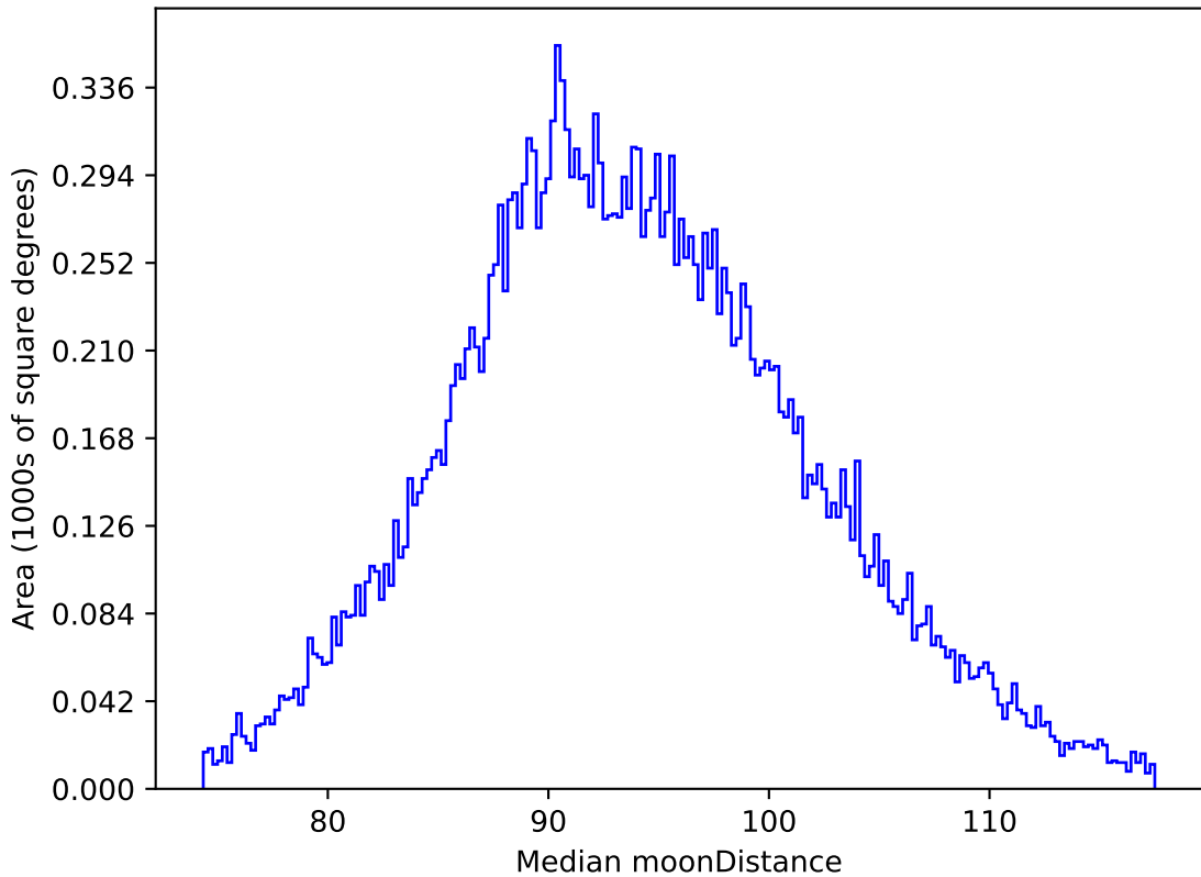
weather_cloudso16v3.4_10yrs All sky i band: Median moonDistance
