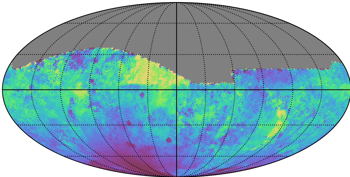
weather_cloudso16v3.4_10yrs All sky g band: Median moonDistance
