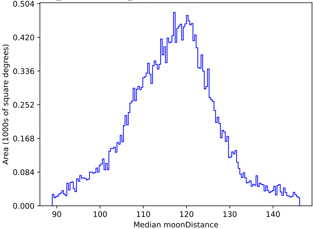
weather_cloudso16v3.4_10yrs All sky g band: Median moonDistance
