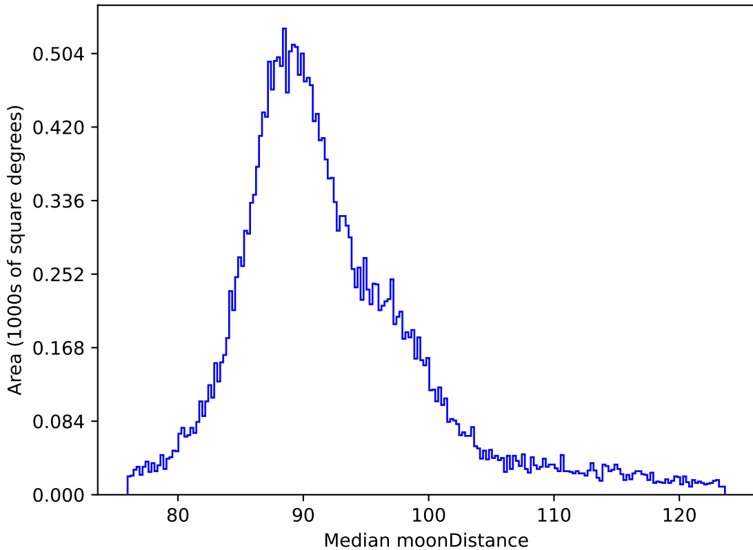
weather_cloudso16v3.4_10yrs All sky all bands: Median moonDistance
