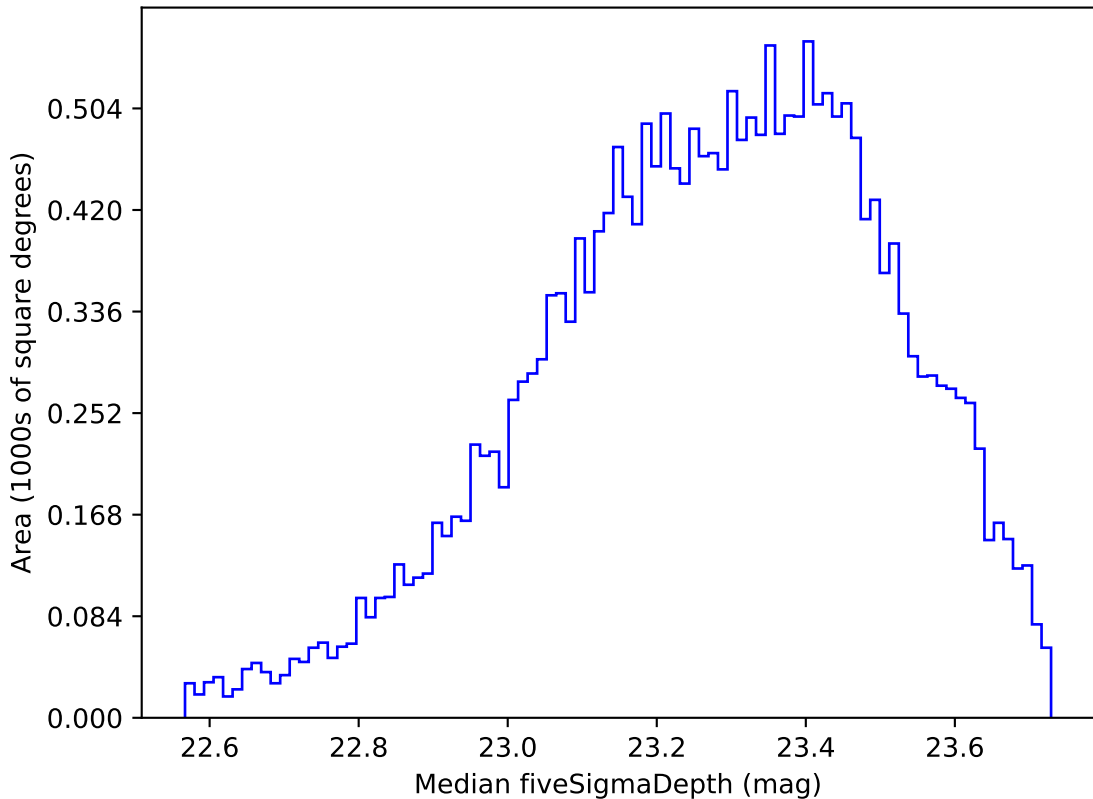
weather_cloudso16v3.4_10yrs Yr 1 u band: Median fiveSigmaDepth
