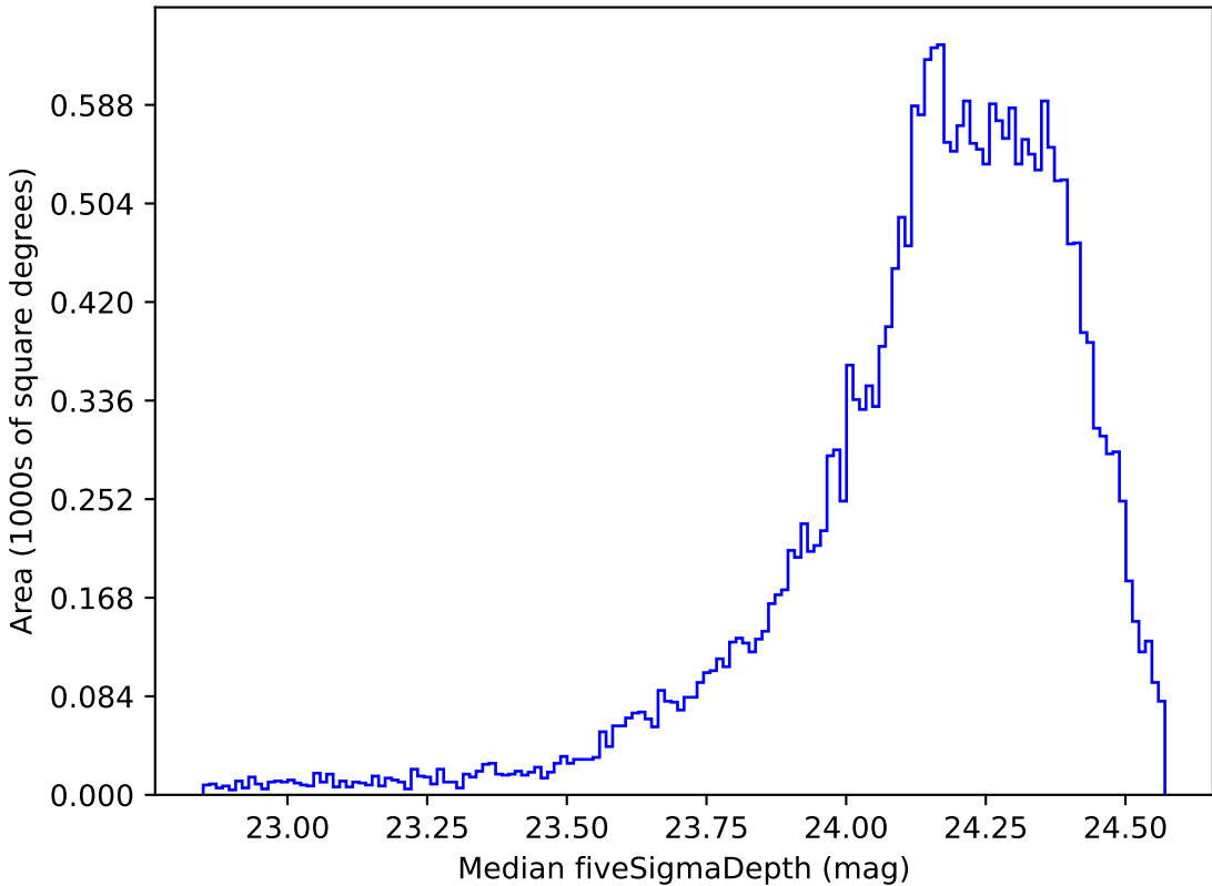
weather_cloudso16v3.4_10yrs Yr 1 r band: Median fiveSigmaDepth
