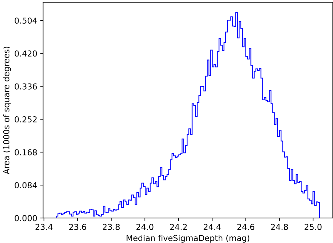
weather_cloudso16v3.4_10yrs Yr 1 g band: Median fiveSigmaDepth
